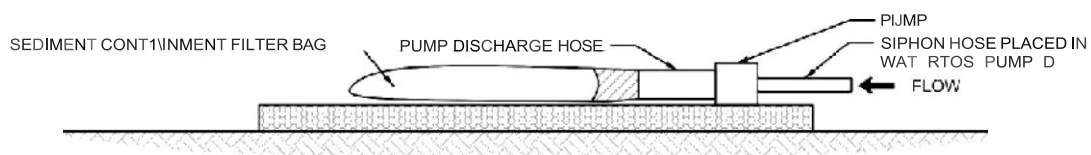
SEDIMENT FILTER BAG PROFILE
