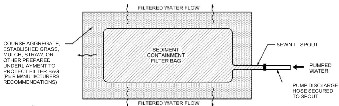
SEDIMENT FILTER BAG PLAN VIEW
